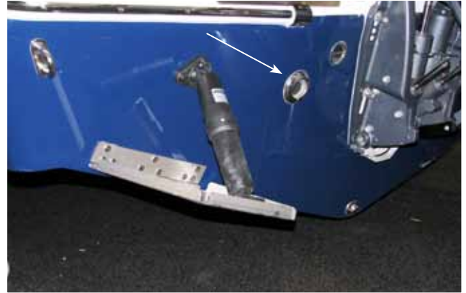
Transom Scupper Drain Check Valve Assembly
